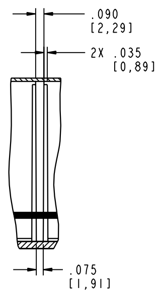
DETAIL C SCALE 2.000
